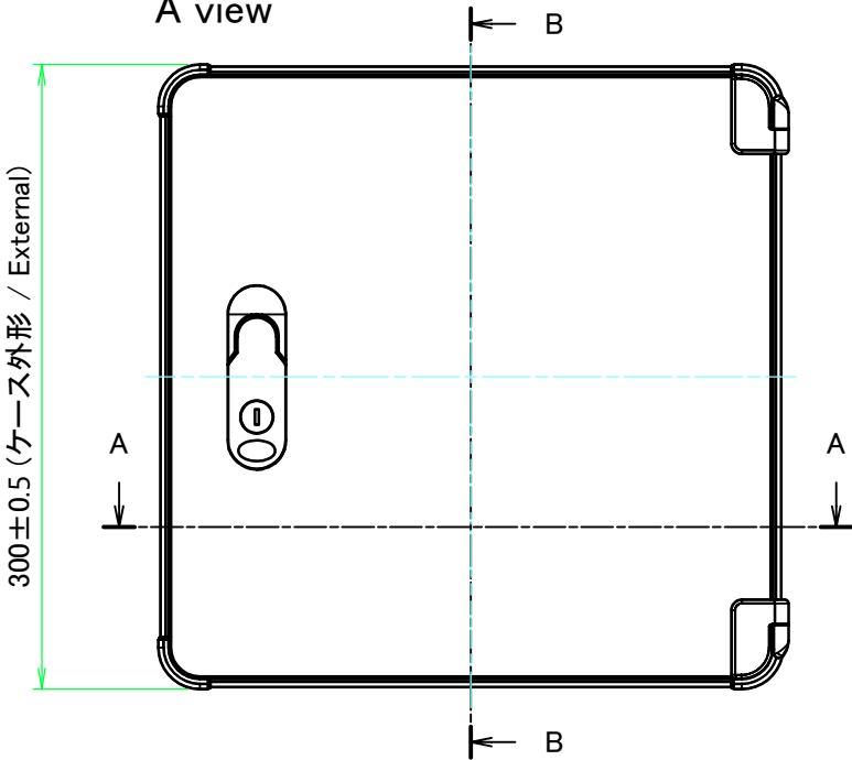
A view
