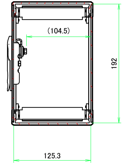
B-B ( 1 :3.5 )
