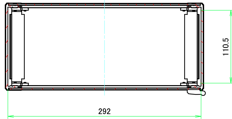
E view
