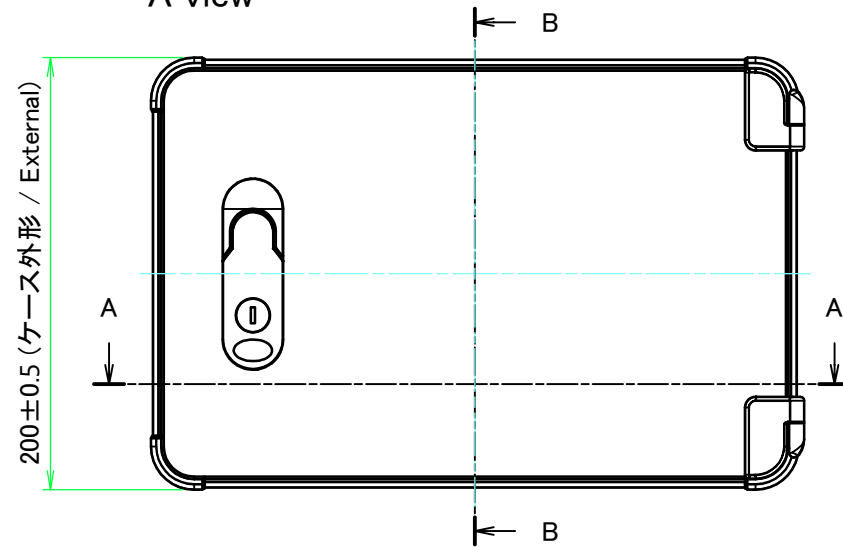
A view
