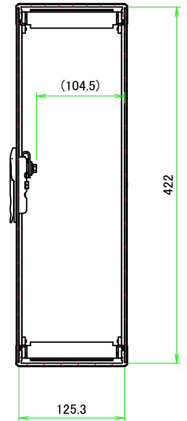
B-B (1:4.5)
