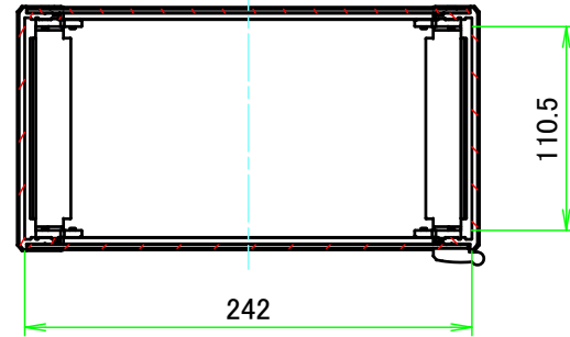
E view
