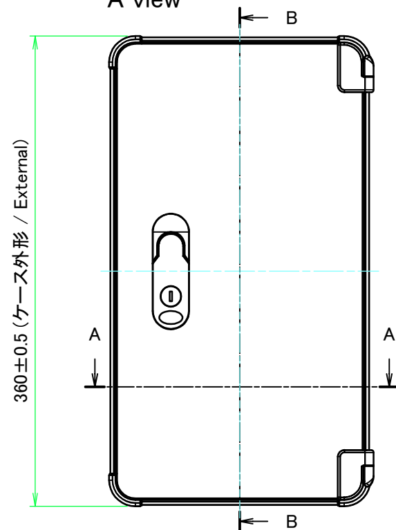
A view
