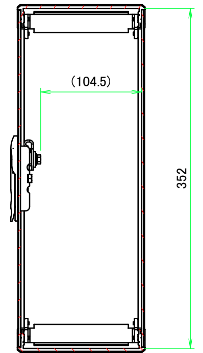
B-B ( 1 :4 )
