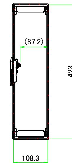
B-B (1:7)
