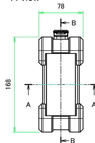
A view
