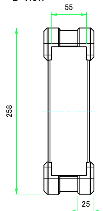
D view
