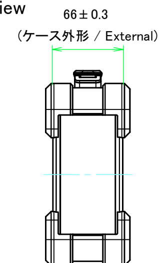
B view
