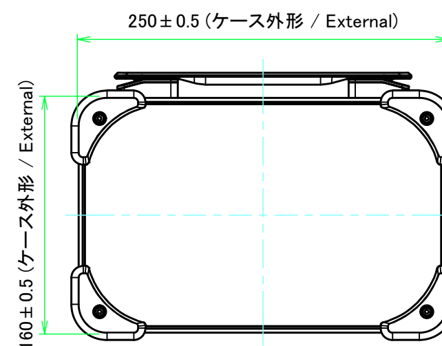
E view
