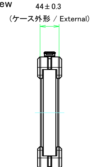
B view
