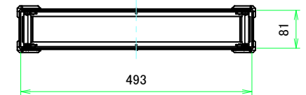
C-C (1:8)
