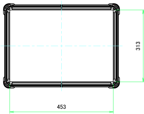
B-B (1:7)
