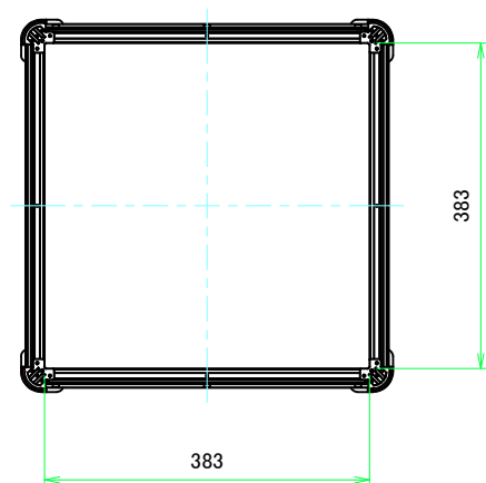
B-B (1:7)
