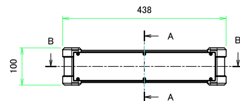
A view
