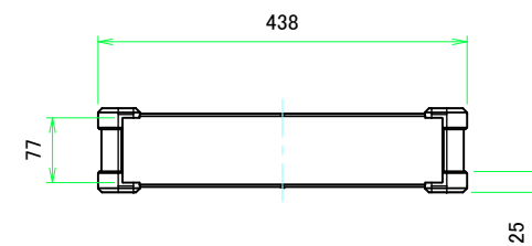
C view
