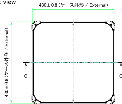
E view
