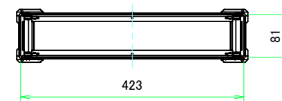
C-C (1:7)
