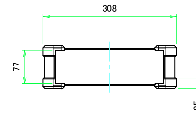
C view
