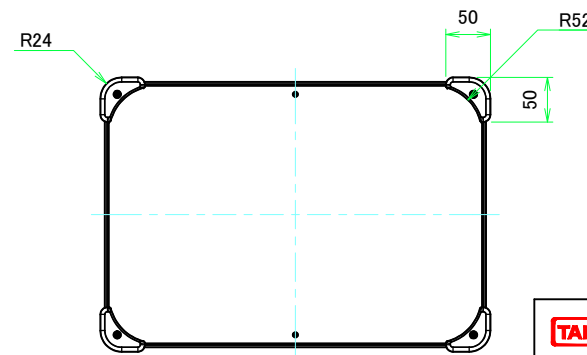
F view
