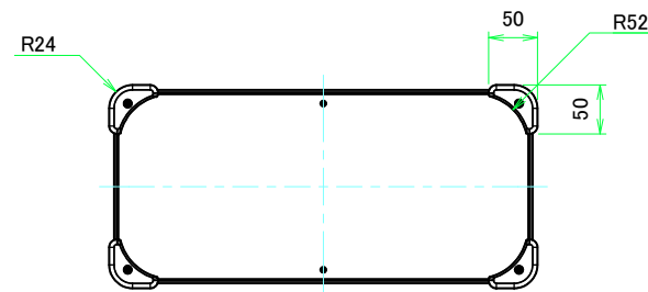
F view
