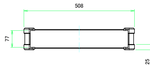
C view
