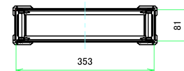
C-C (1:7)
