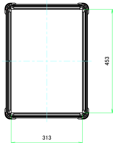
B-B (1:7)
