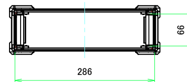
A-A (1:5.5)
