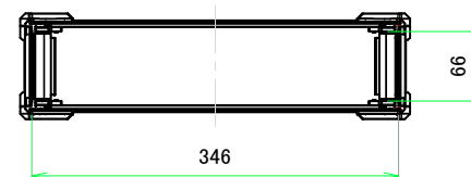
A-A (1:5.5)
