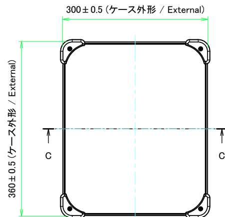
E view
