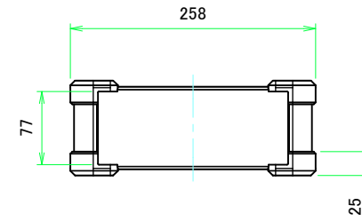
C view
