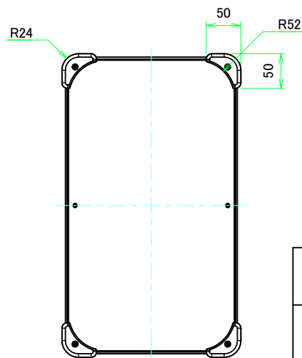
F view
