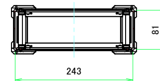
C-C (1:5.5)
