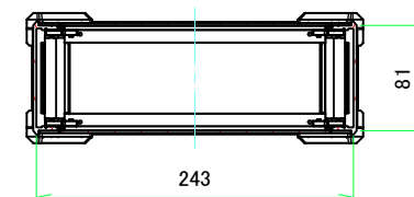
C-C (1:4.5)
