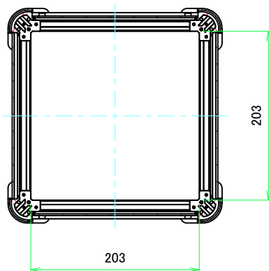
B-B (1:4.5)
