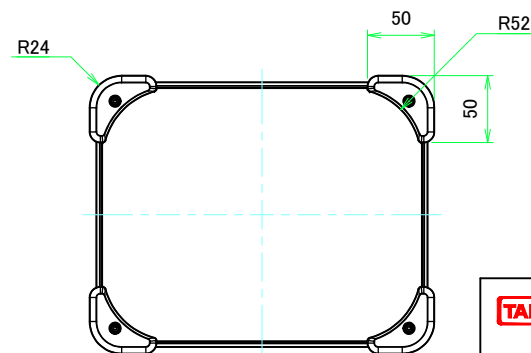
F view
