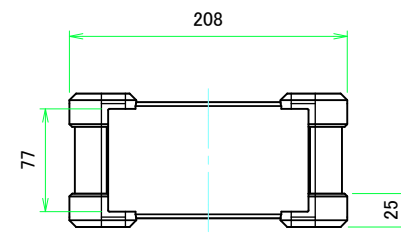
C view
