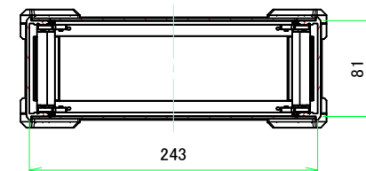
C-C (1:4)
