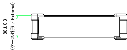
D view
