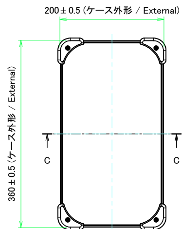
E view
