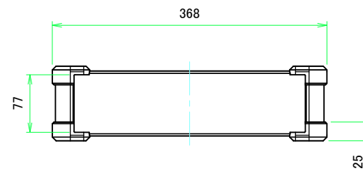
C view
