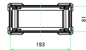
C-C (1:5)
