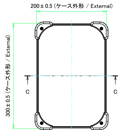
E view
