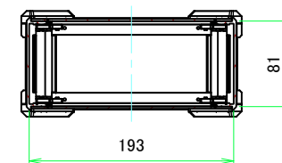
C-C (1:4.5)
