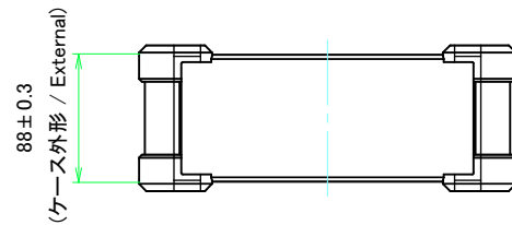
D view
