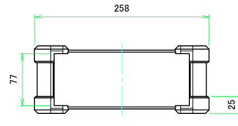
C view
