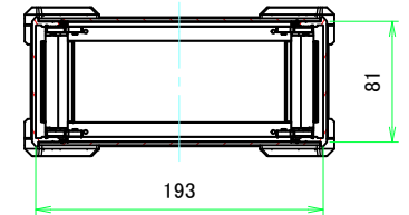
C-C (1:4)
