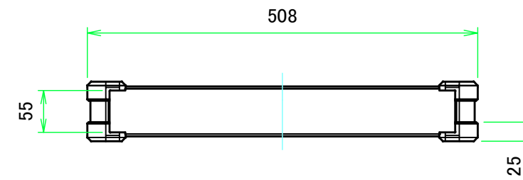
C view
