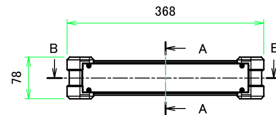
A view
