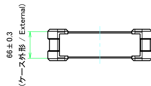
D view
