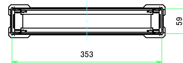
C-C ( 1:5.5 )
