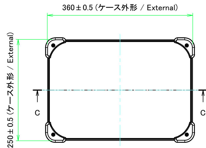
E view
