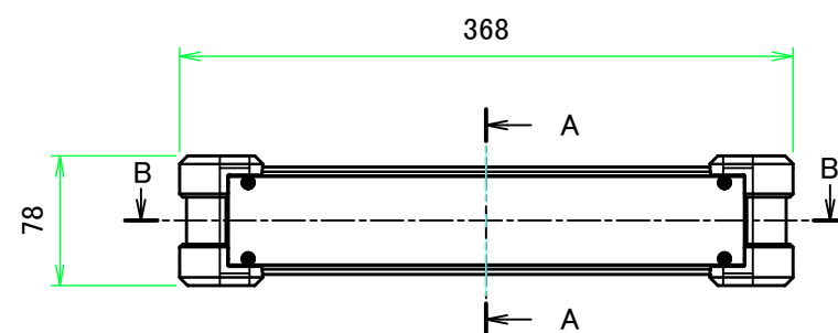
A view
