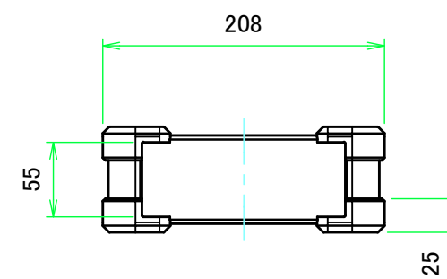
C view
