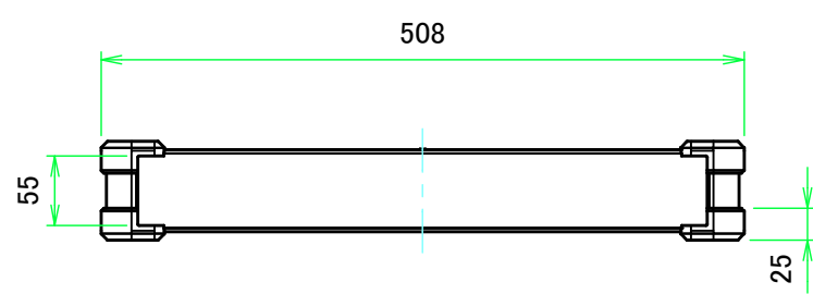
C view
