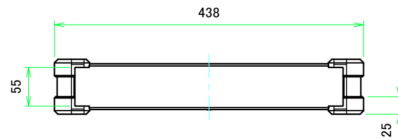
C view
