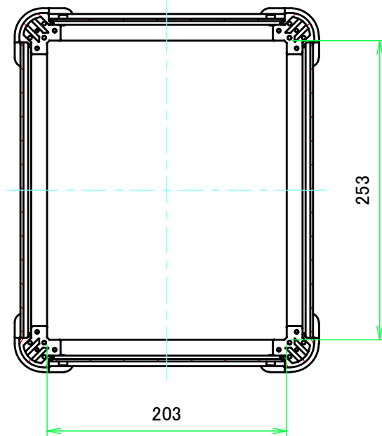
D view
