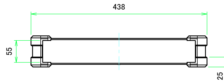
C view
