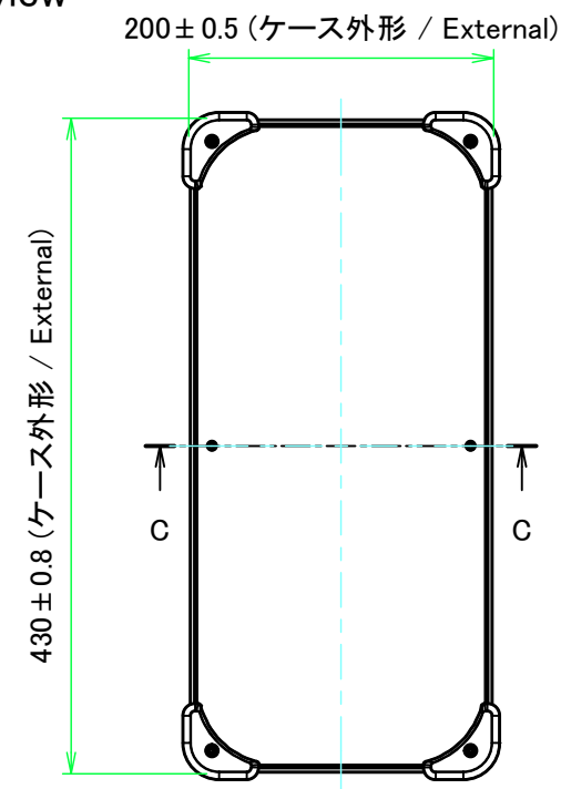
E view
