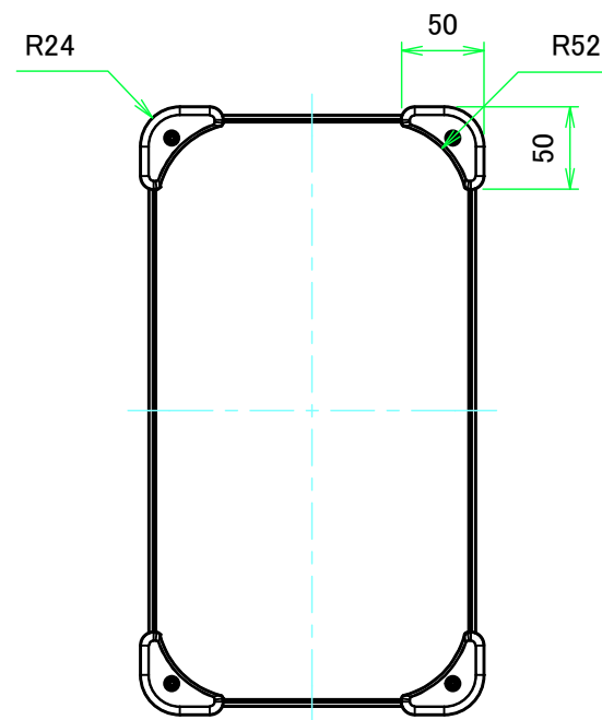
F view
