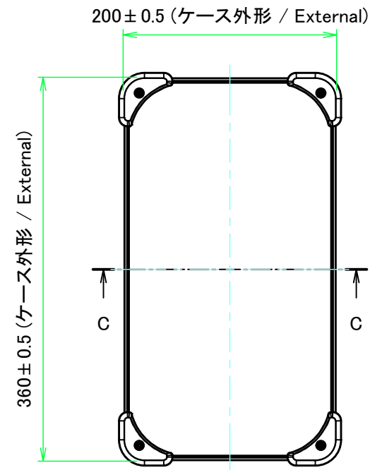
E view
