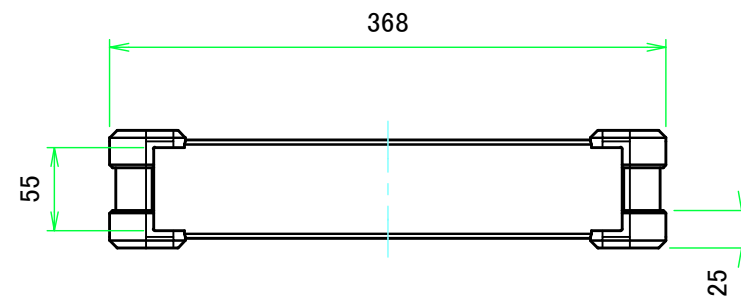
C view
