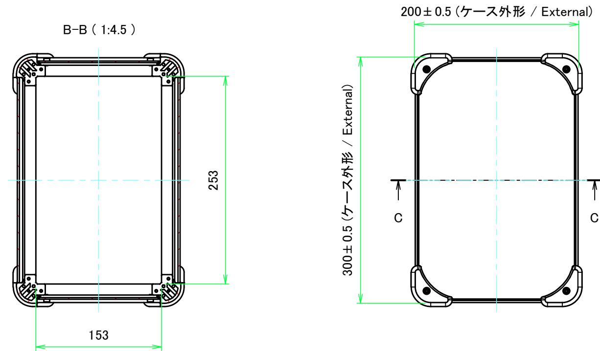
E view
