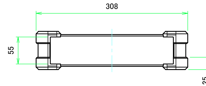
C view
