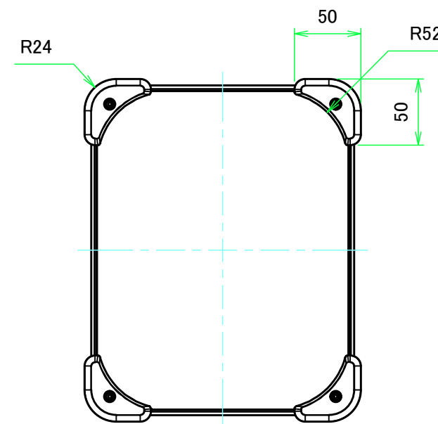
F view
