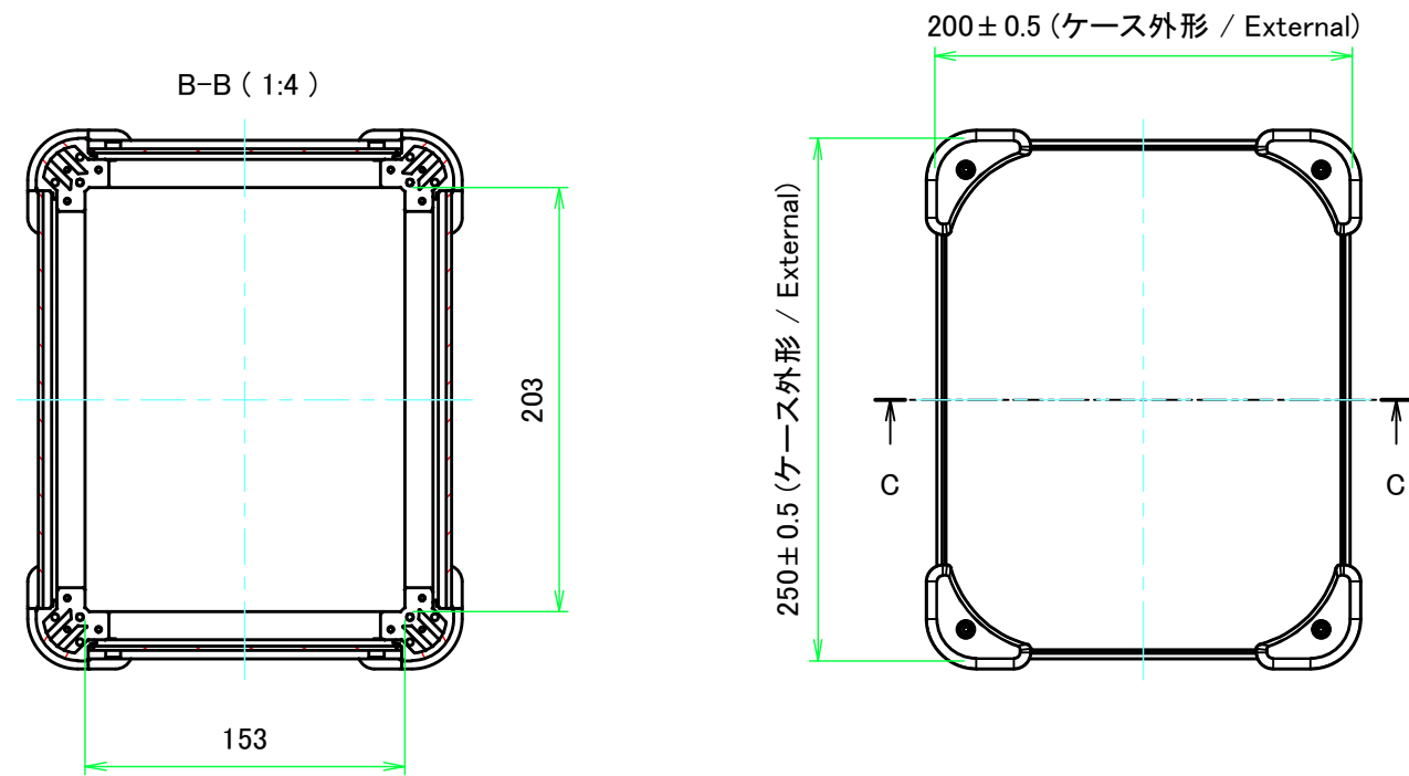
E view
