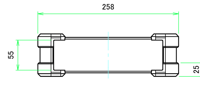
C view
