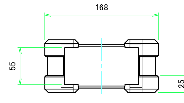
C view
