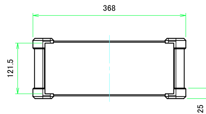
C view
