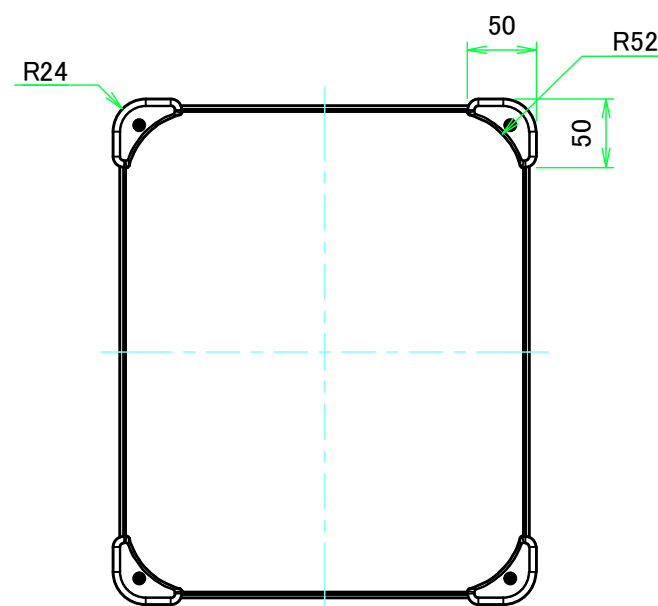
F view
