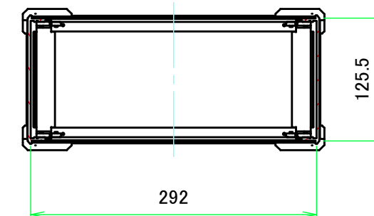
C-C ( 1:5.5 )
