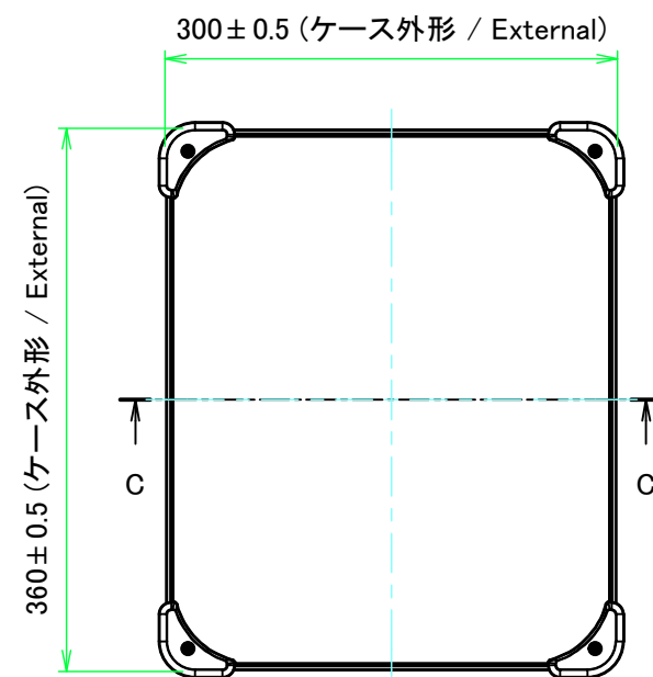
E view
