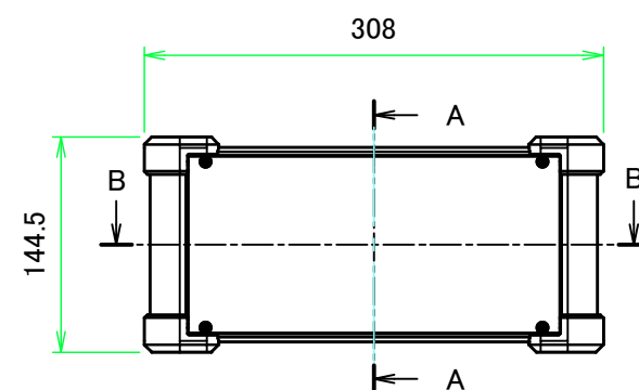
A view
