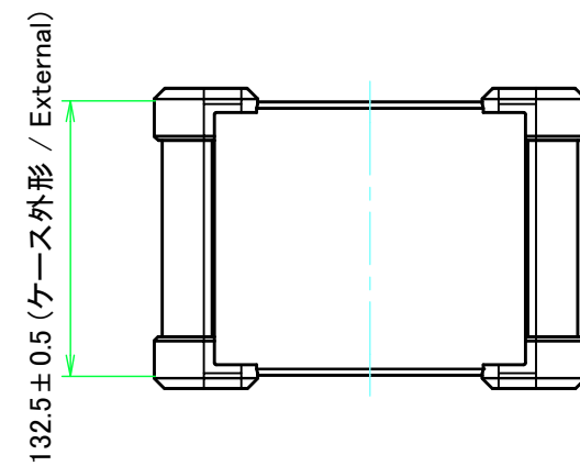
D view
