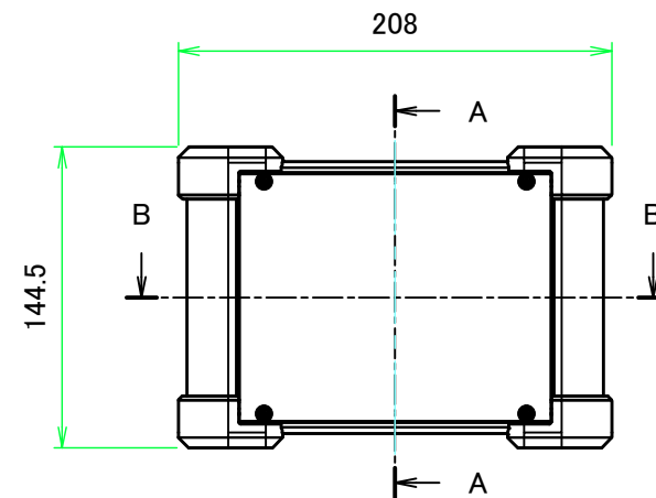
A view
