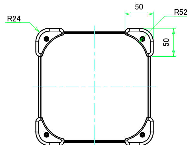
F view
