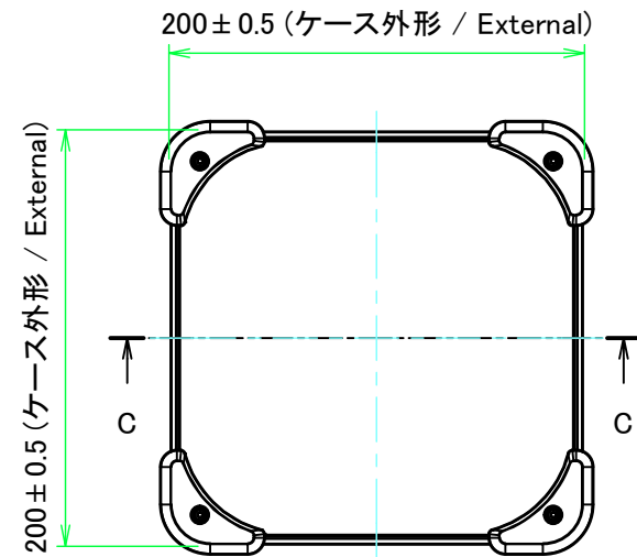
E view
