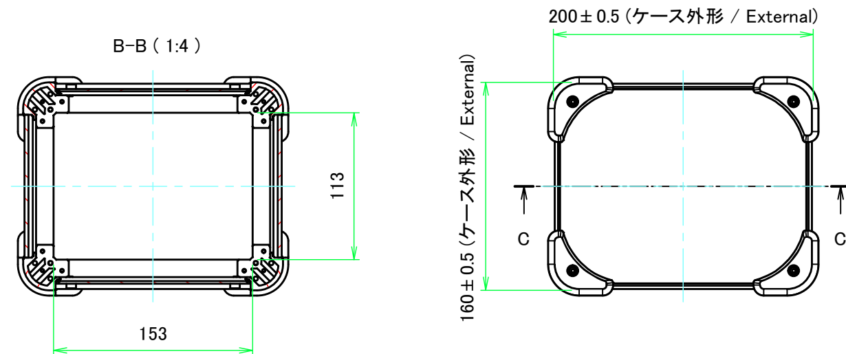
E view
