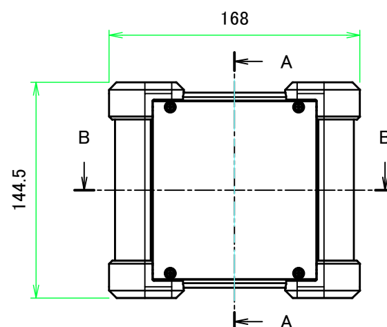
A view
