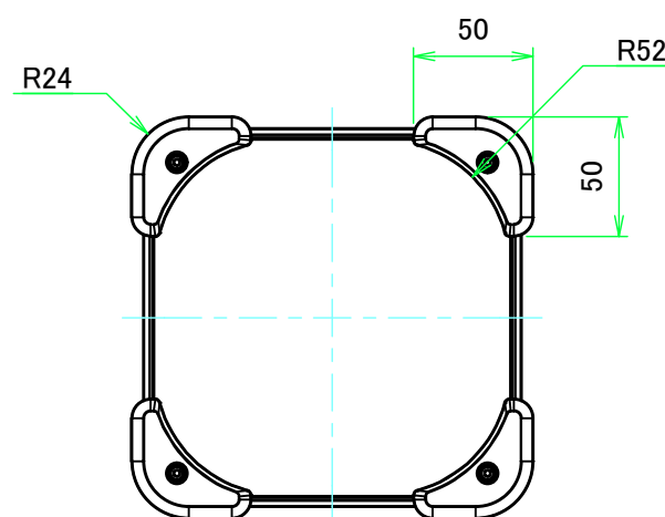
F view
