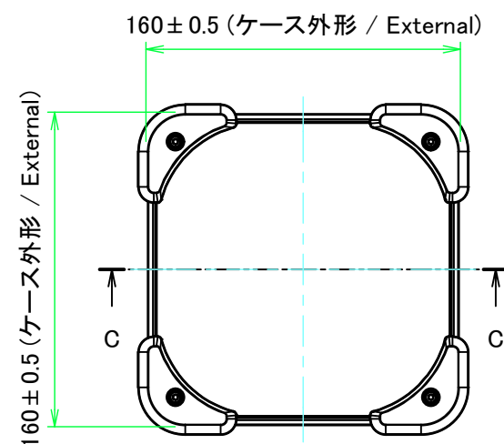
E view
