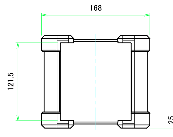
C view
