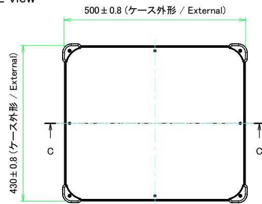
E view
