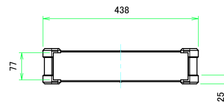
C view
