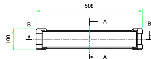
A view
