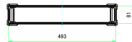
C-C (1:7)
