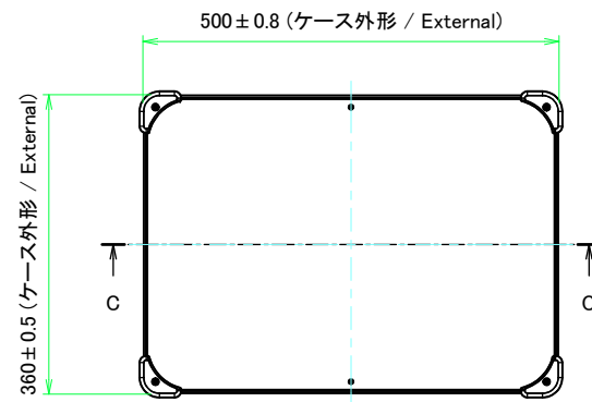
E view
