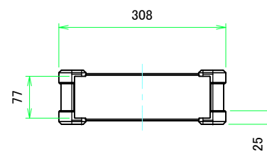
C view
