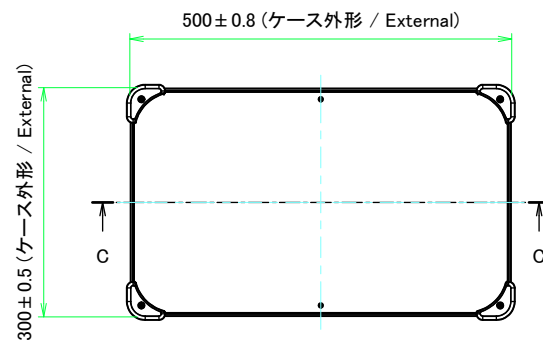
E view
