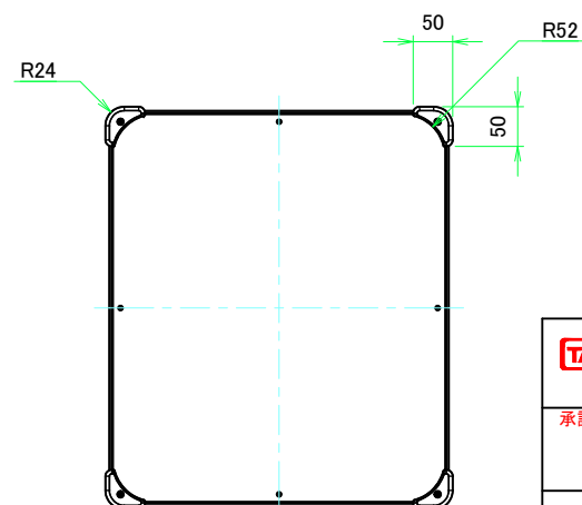
F view
