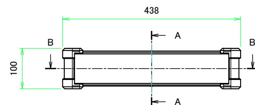
A view
