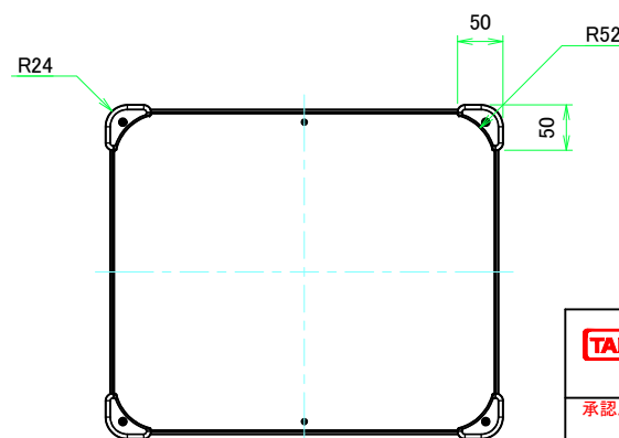
F view
