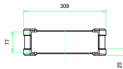
C view
