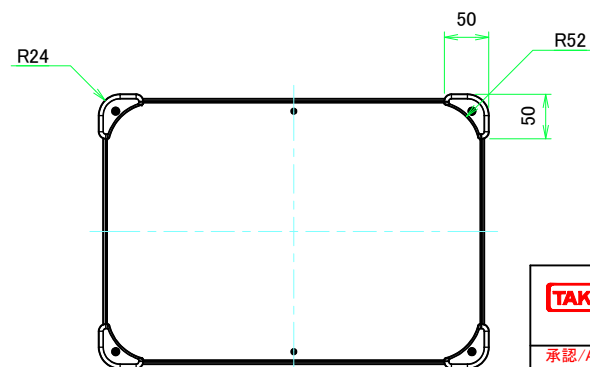
F view
