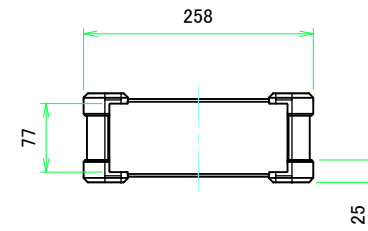
C view
