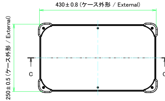
E view
