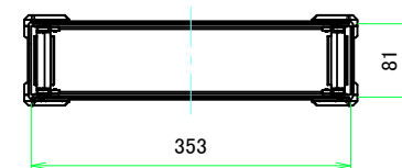
C-C (1:6.5)
