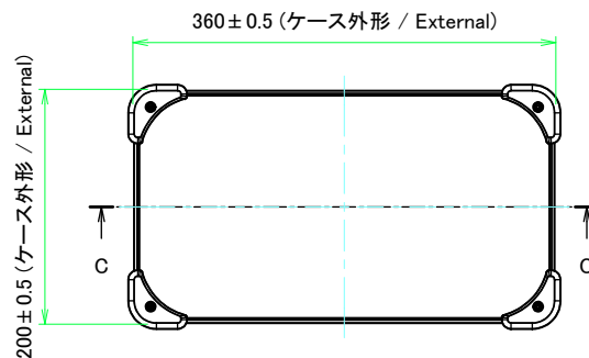
E view
