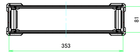
C-C (1:5)
