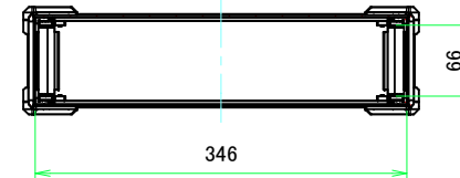
A-A (1:5.5)
