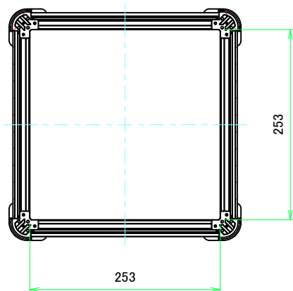
B-B (1:5)
