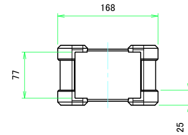
C view
