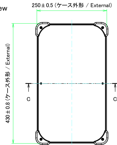
A view
